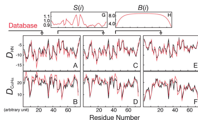
Figure 3. Flowchart of the seq2rdc approach. The sequence of ubiquitin and D_{\text{NH}} (A, C, E) and D_{\text{CaH}\alpha} (B, D, F) are simulated as examples. Black lines represent the simulation from the LAW, and red lines from seq2rdc . A and B) database only; C and D) corrected with the scaling factor S(i) depending on the composition of residues i-7 to i-2 and i+2 to i+7 (G); E and F) corrected with a length-dependent hyperbolic baseline B(i) (H).
